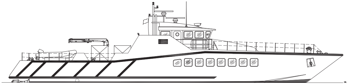
Outboard Profile
