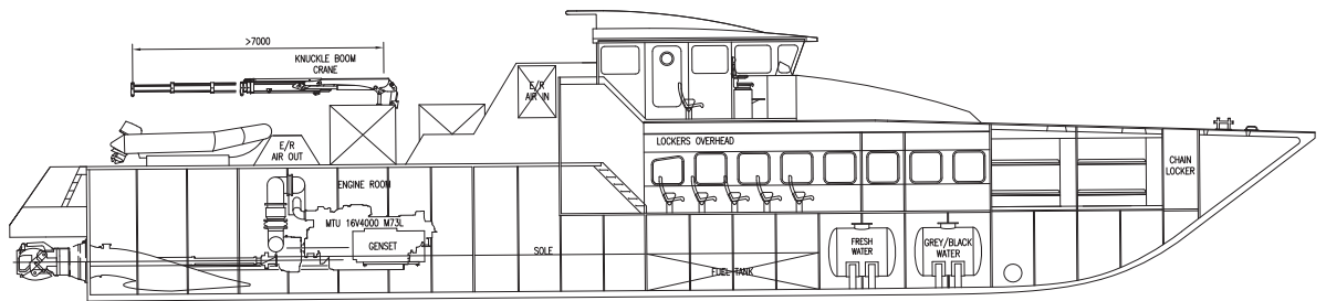
Inboard Profile
